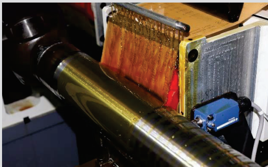
Superfinishing by Film Backed Abrasives
